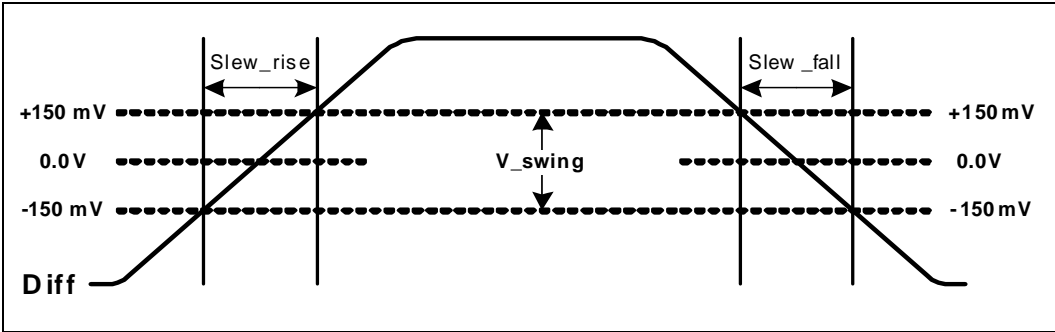
Figure 2-5. Differential Measurements
