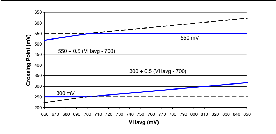
Figure 2-5. Differential Measurements
