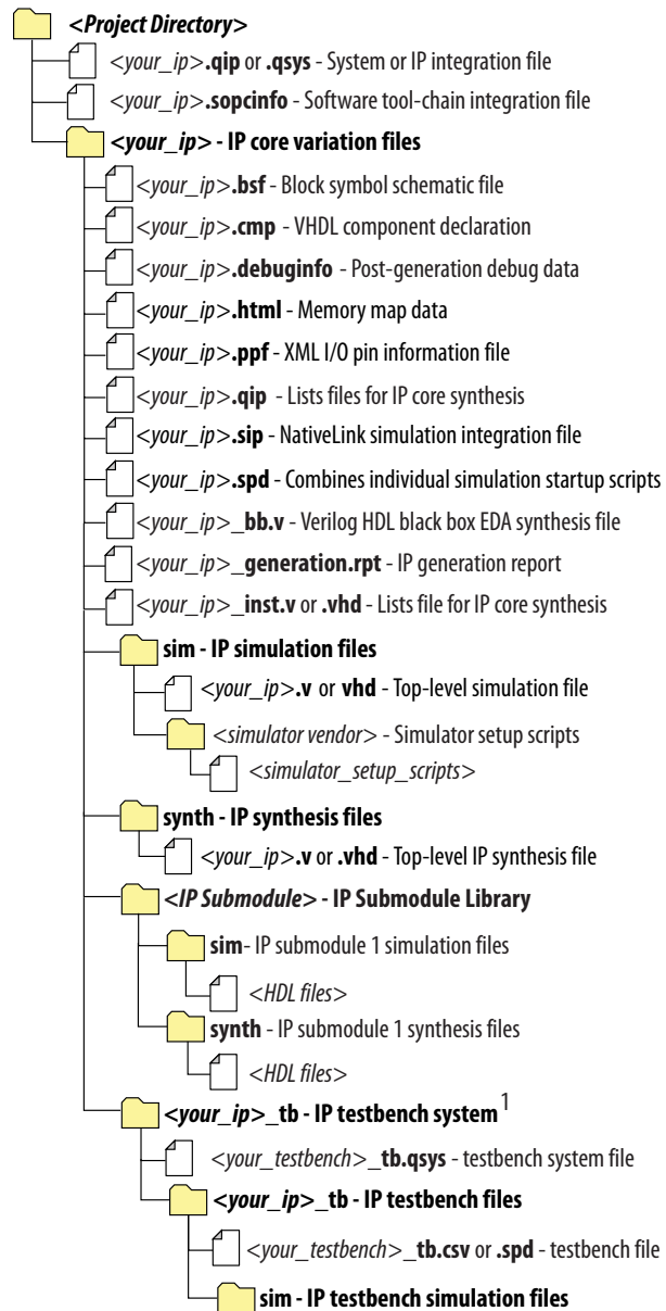
Figure 2-4: Files generated for IP cores and Qsys Systems
