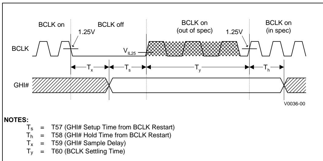
Figure 16. Intel SpeedStep Technology/Deep Sleep Timing
