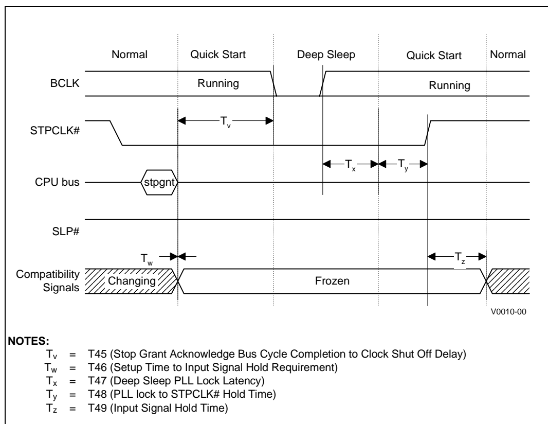
Figure 14. Quick Start/Deep Sleep Timing
