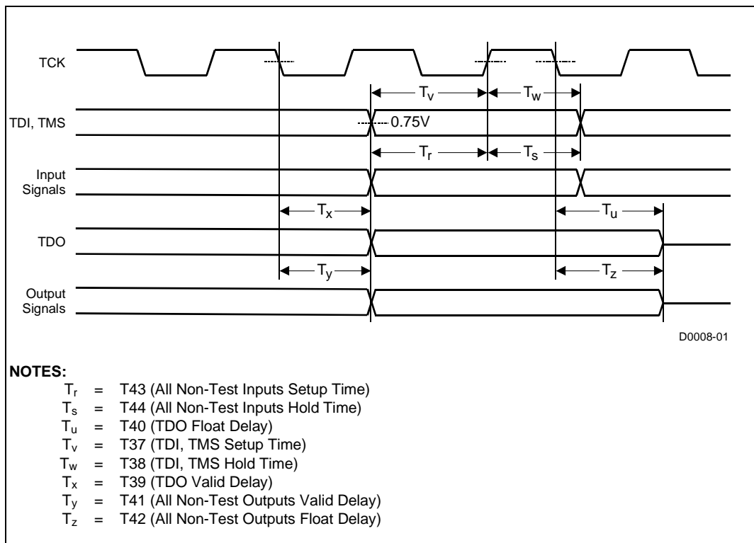
Figure 12. Test Timings (Boundary Scan)
