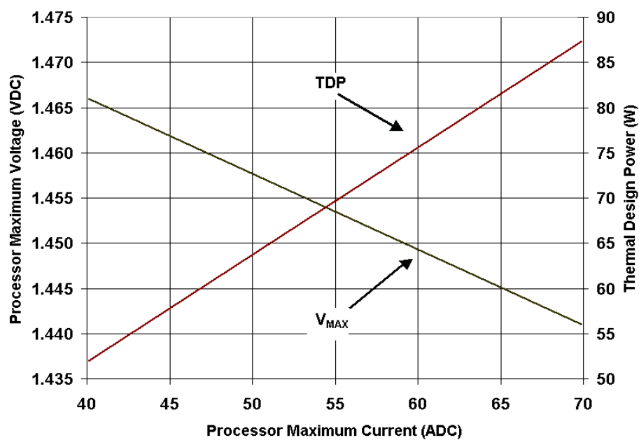
Figure 19. Processor Thermal Design Power vs Electrical Projections for VID = 1.500V
