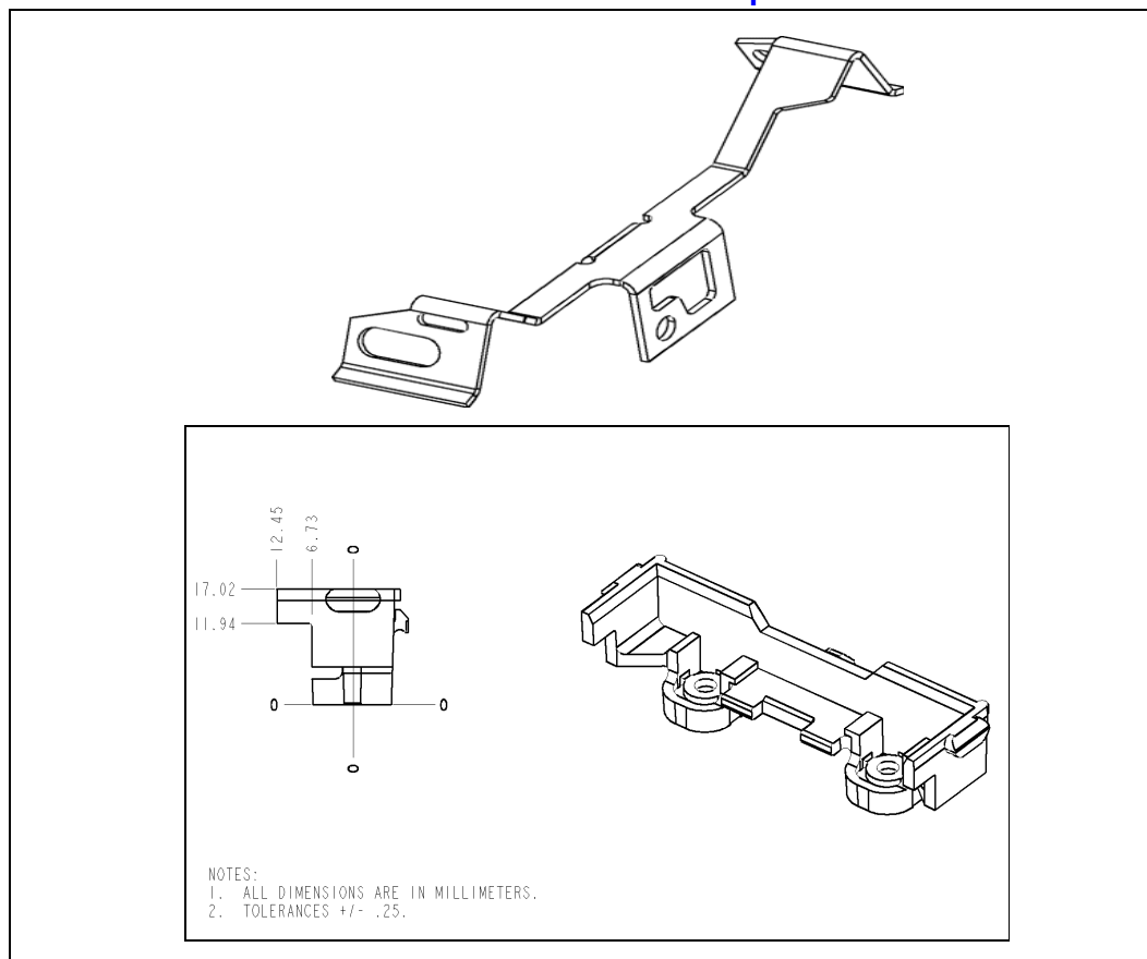
Figure 24. Boxed Processor Retention Mechanism and Clip
