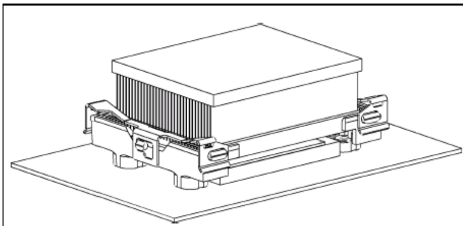
Figure 31. Assembled View of the 1U Thermal Solution
