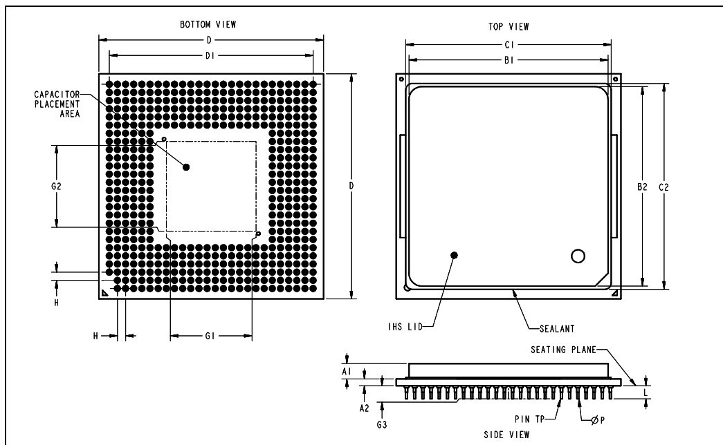
Figure 28. Processor Package
