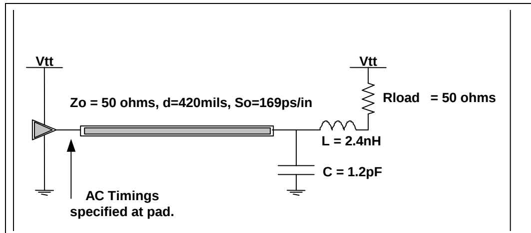
Figure 5. Electrical Test Circuit
