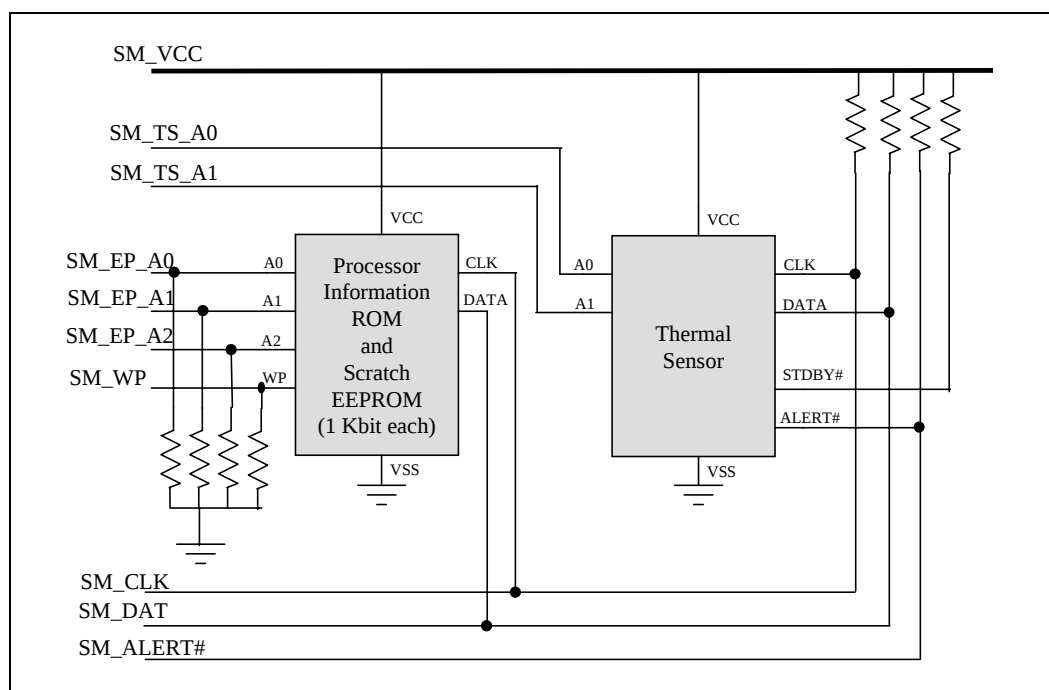
Figure 42. Logical Schematic of SMBus Circuitry
