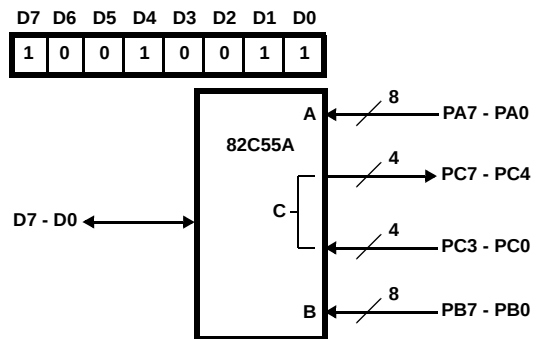
CONTROL WORD #11
