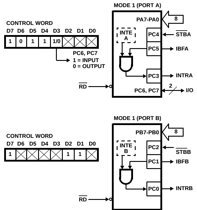
FIGURE 6. MODE 1 INPUT
