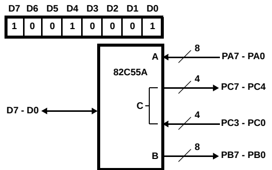
CONTROL WORD #9
