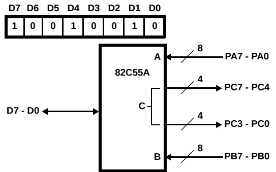
CONTROL WORD #10
