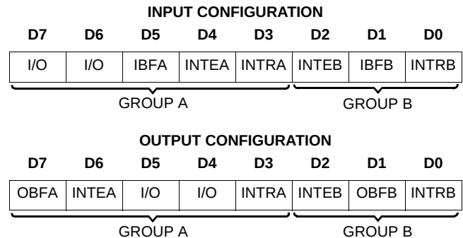
FIGURE 15. MODE 1 STATUS WORD FORMAT
