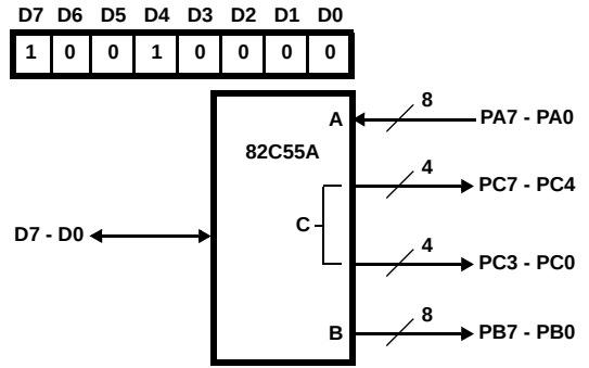
CONTROL WORD #8
