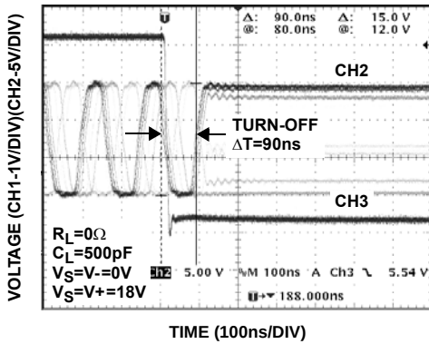
FIGURE 9. TURN-OFF (TRI)
