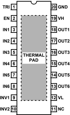
EL5001 (20-PIN HSSOP) TOP VIEW
