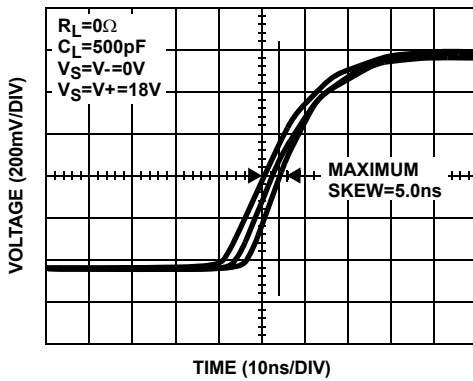
FIGURE 13. SKEW
