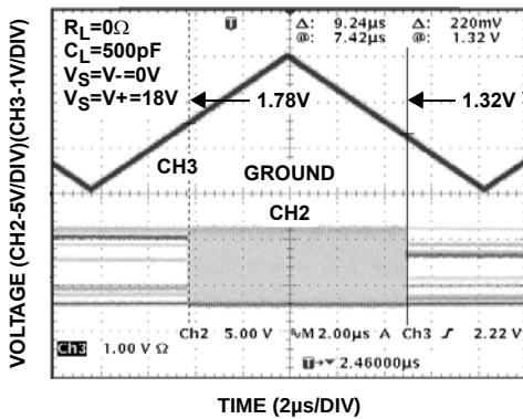
FIGURE 11. ENABLE/DISABLE THRESHOLD
