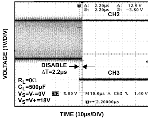
FIGURE 7. DISABLE RESPONSE
