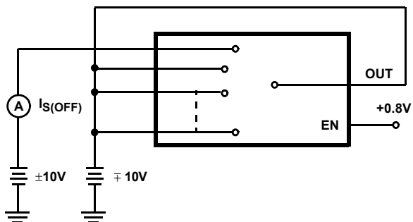
FIGURE 2C. I_{\text{S(OFF)}} TEST CIRCUIT (NOTE 9)
