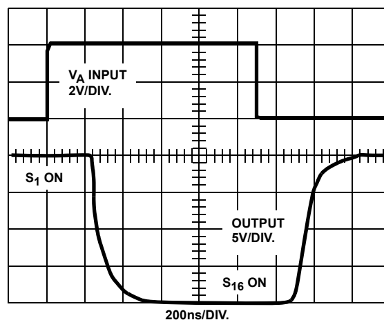
FIGURE 6D. WAVEFORMS
