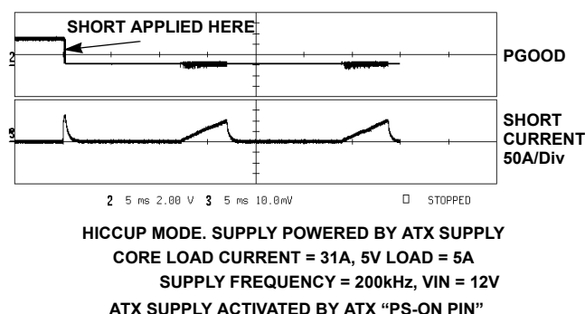
FIGURE 8. SHORT APPLIED TO SUPPLY AFTER POWER-UP
