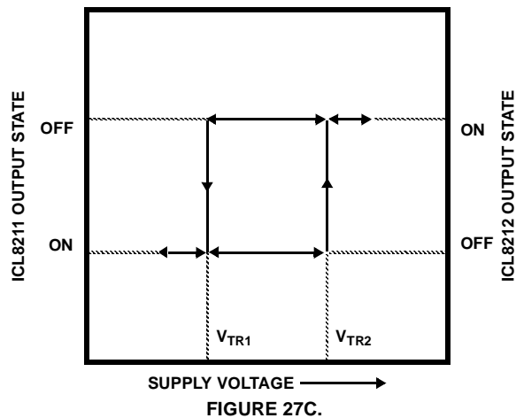
FIGURE 27. TWO ALTERNATIVE VOLTAGE DETECTION CIRCUITS EMPLOYING HYSTERESIS TO PROVIDE PAIRS OF WELL DEFINED TRIP VOLTAGES
