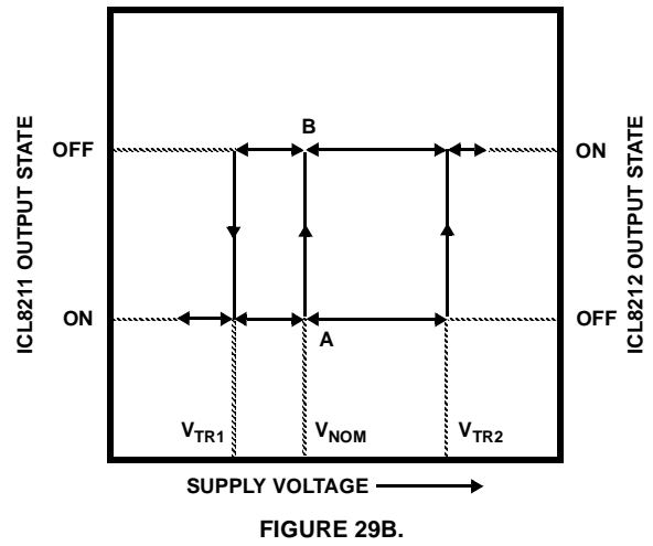
FIGURE 29. NON-VOLATILE LOW VOLTAGE INDICATOR
