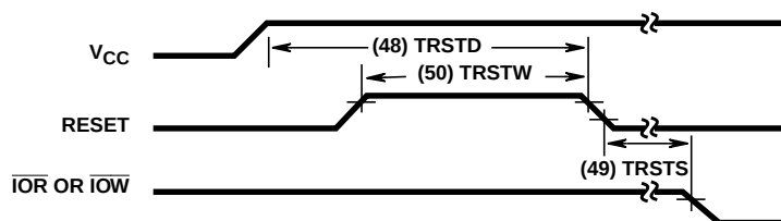
FIGURE 14. RESET
