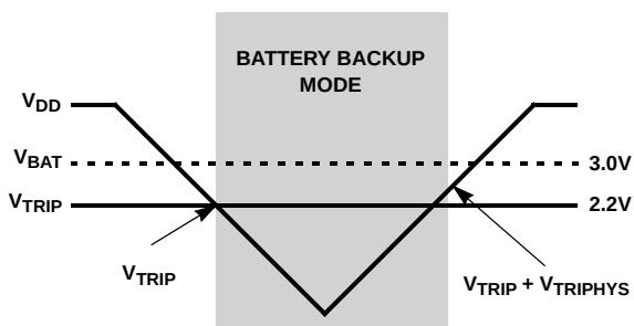
FIGURE 14. BATTERY SWCHOVER WHEN V_{BAT} > V_{TRIP}
