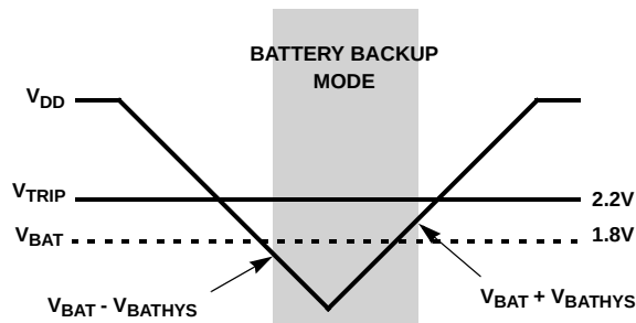
FIGURE 13. BATTERY SWCHOVER WHEN V_{BAT} < V_{TRIP}
