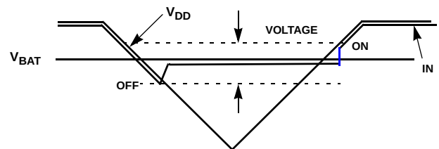
FIGURE 15. BATTERY SWCHOVER IN LEGACY MODE
