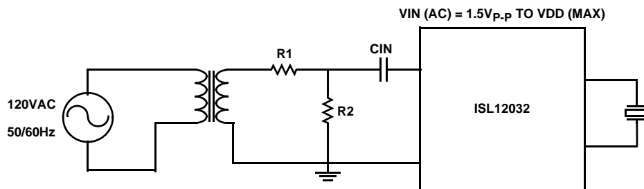
FIGURE 11. AC INPUT USING A TRANSFORMER SECONDARY
