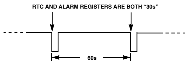
FIGURE 5. \overline{\text{IRQ}} WAVEFORM
