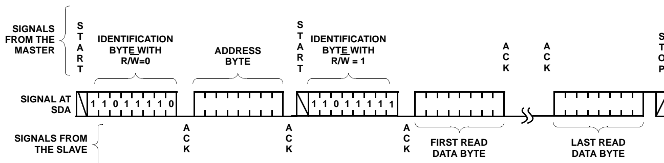
FIGURE 9. SLAVE ADDRESS, WORD ADDRESS, AND DATA BYTES
