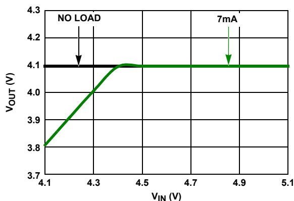
FIGURE 33. DROPOUT, ISL21080-41
