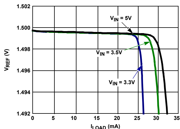
FIGURE 36. DIFFERENT V_{IN} AT HIGH TEMPERATURE (+85°C)
