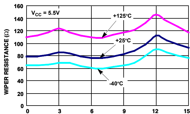
FIGURE 1. WIPER RESISTANCE vs TAP POSITION [ I(RW) = V_{CC}/R_{TOTAL} ] FOR 10k\Omega (W)
