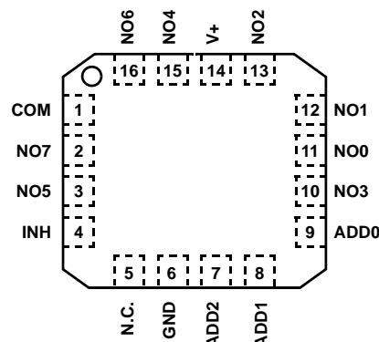
ISL84781IR (3x3 THIN QFN) TOP VIEW
