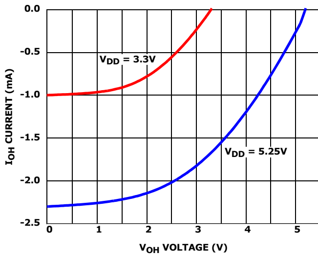
FIGURE 17. I_{OH} vs V_{OH} vs V_{DD} for \overline{INT} and \overline{ALM}
