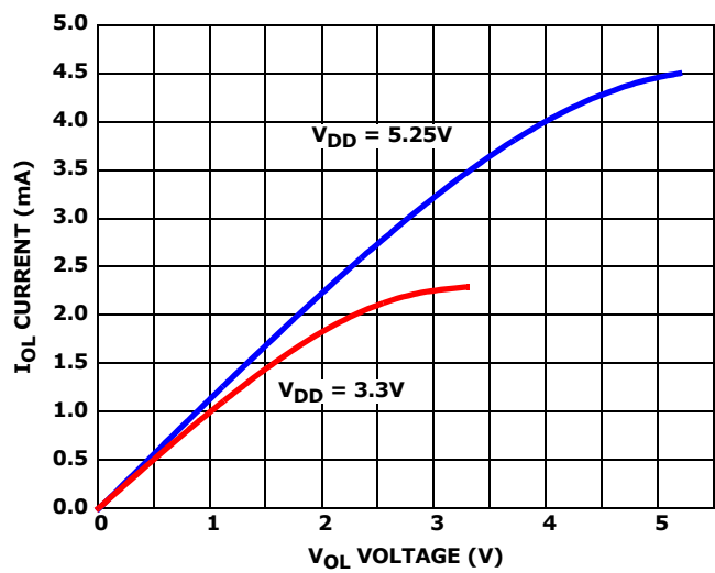
FIGURE 18. I_{OL} vs V_{OL} vs V_{DD} for \overline{INT} and \overline{ALM}
