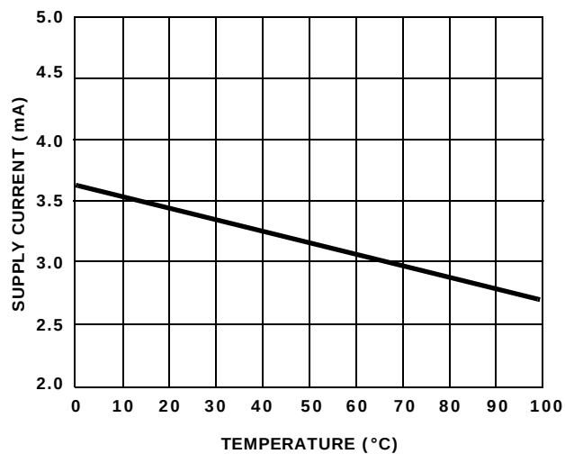
FIGURE 3. V_{DD} BIAS CURRENT
