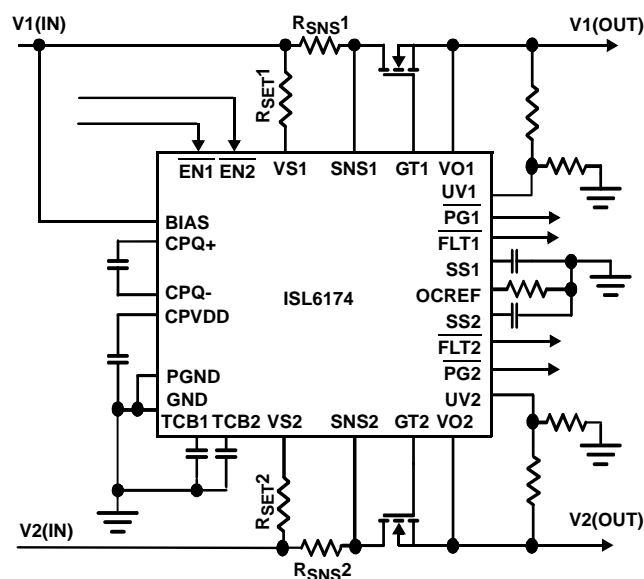
FIGURE 1. TYPICAL APPLICATION
