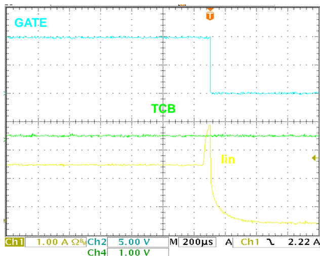
FIGURE 21. WOC CIRCUIT BREAKER OPERATION ZOOM
