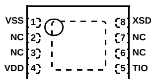
ISL6296 (8 LD 2X3 TDFN) TOP VIEW
