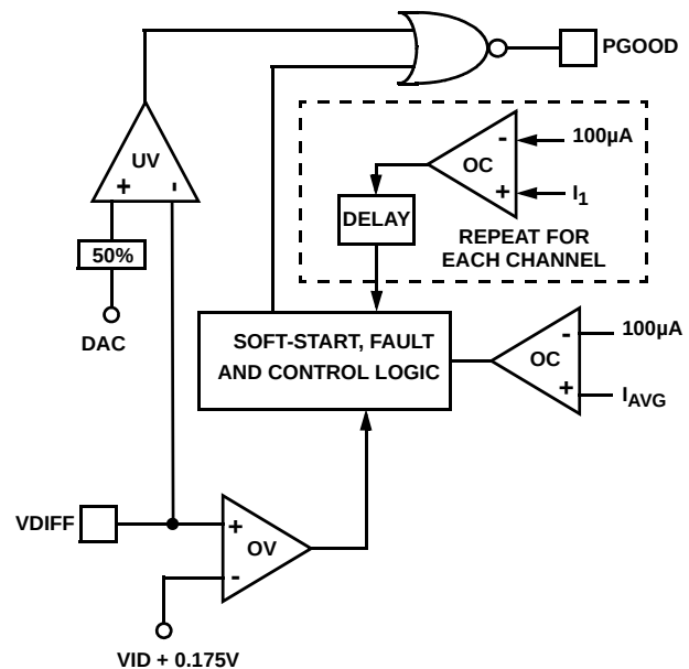
FIGURE 12. POWER GOOD AND PROTECTION CIRCUITRY
