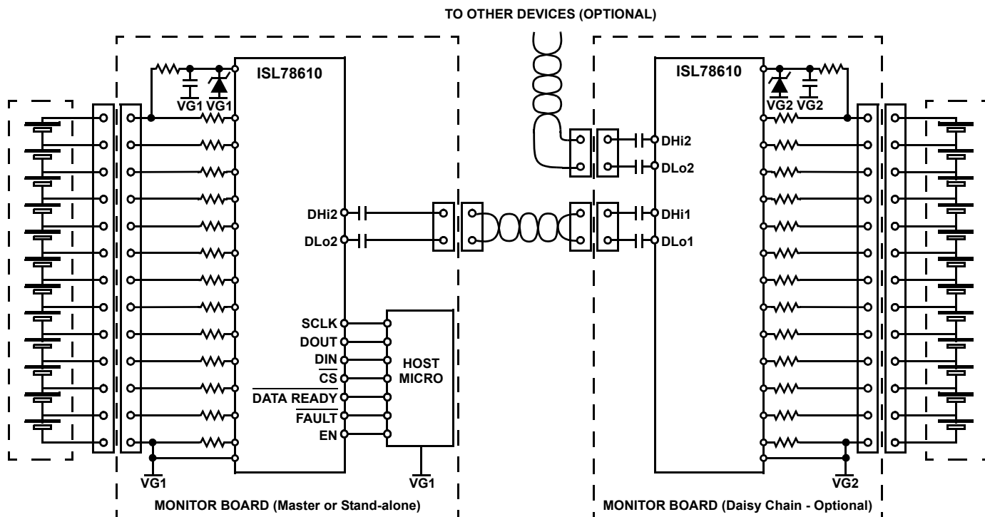
FIGURE 1. TYPICAL APPLICATION
