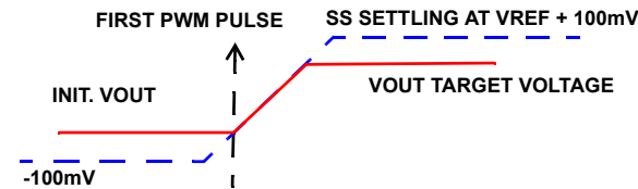
FIGURE 27. SOFT-START WITH V_{OUT} < \text{TARGET VOLTAGE}
