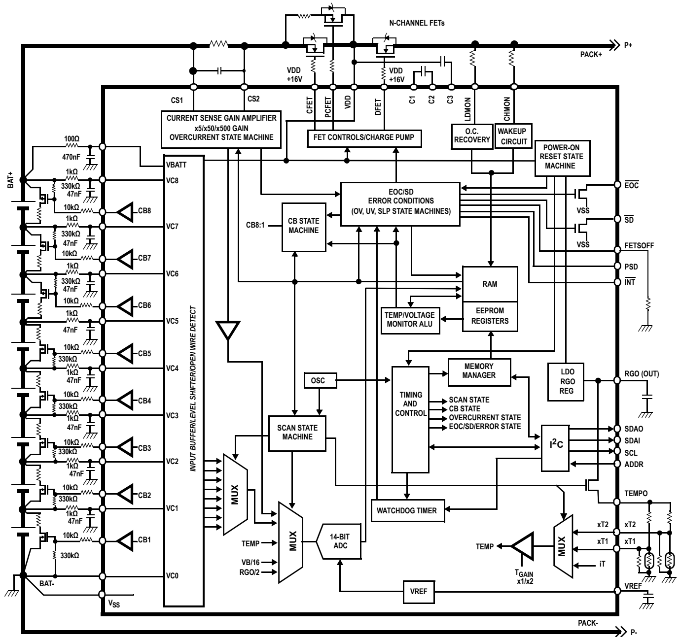
FIGURE 2. BLOCK DIAGRAM
