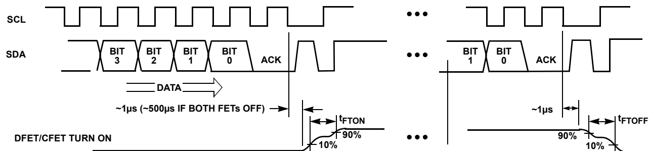
FIGURE 6. I²C FET CONTROL TIMING
