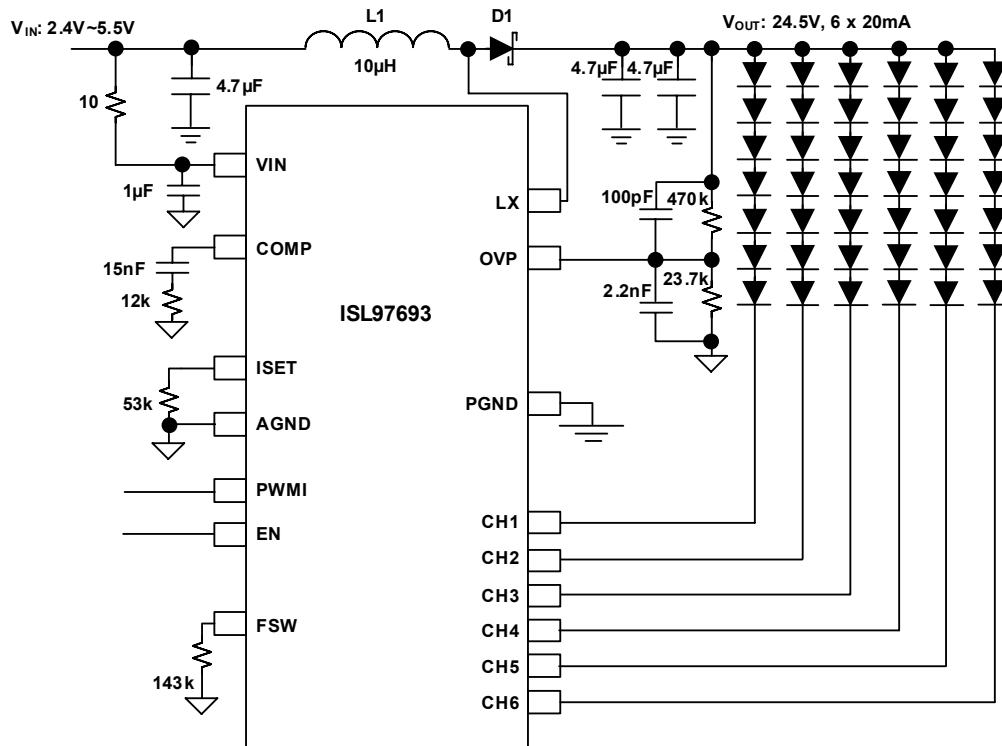
FIGURE 4. ISL97693 TYPICAL APPLICATION DIAGRAM
