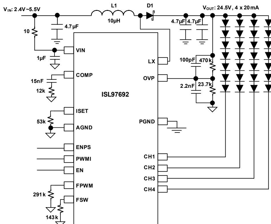
FIGURE 3. ISL97692 TYPICAL APPLICATION DIAGRAM
