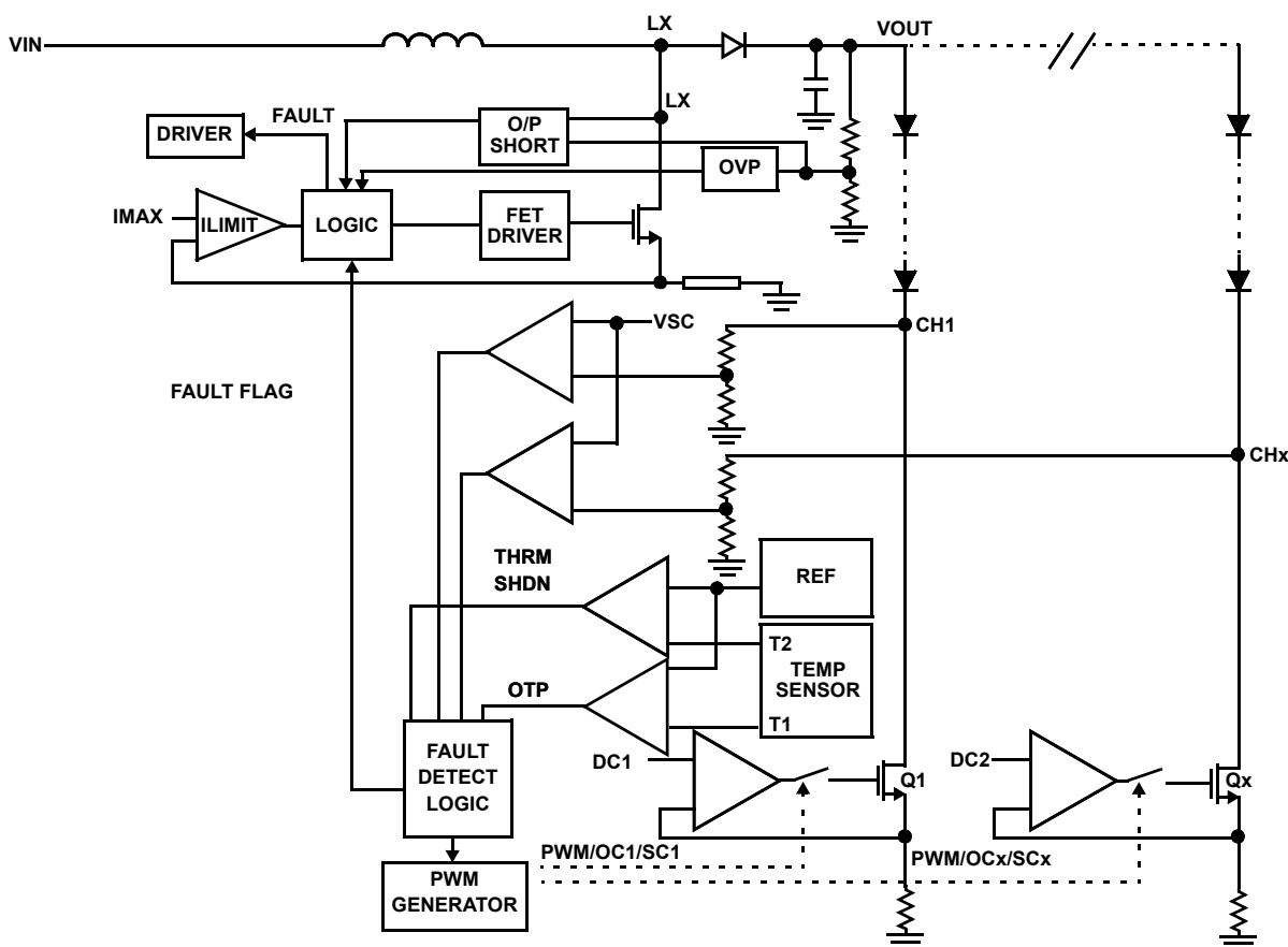
FIGURE 35. ISL97692/3/4A SIMPLIFIED FAULT PROTECTIONS
