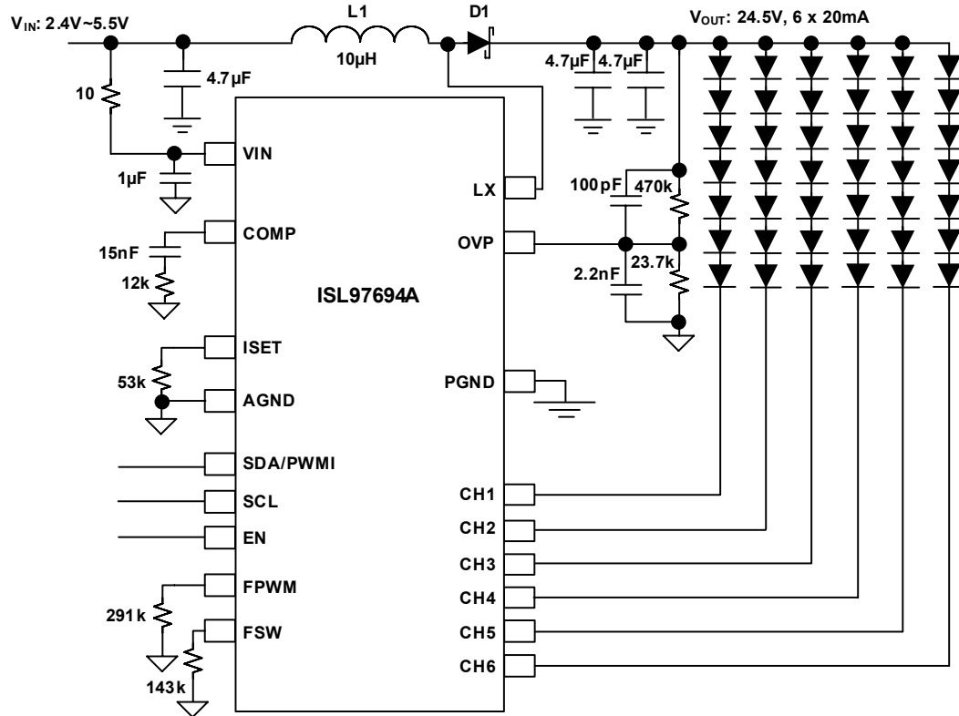
FIGURE 5. ISL97694A TYPICAL APPLICATION DIAGRAM
