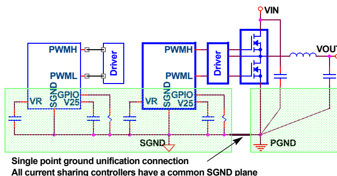
FIGURE 23. COMMON SGND PLANE FOR CURRENT SHARING
