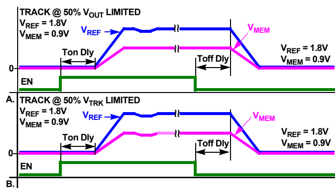
FIGURE 19. RATIOMETRIC TRACKING
