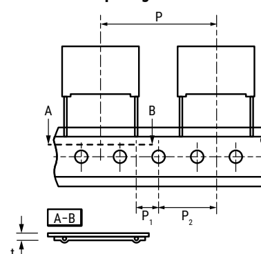
Lead Spacing 22.5 & 27.5 mm
