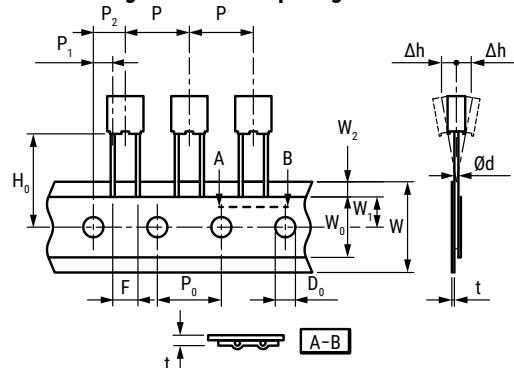
Figure 1 – Lead Spacing 7.5 mm
