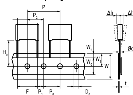
Lead Spacing 10 & 15 mm
