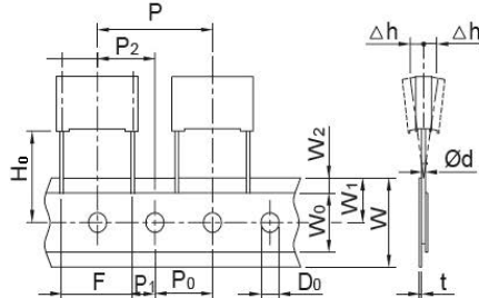
Lead Spacing 10 &amp; 15 mm
