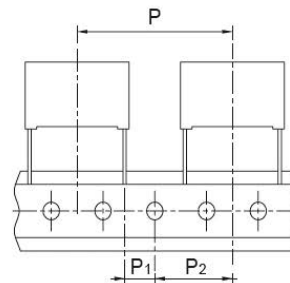
Lead Spacing 22.5 &amp; 27.5
