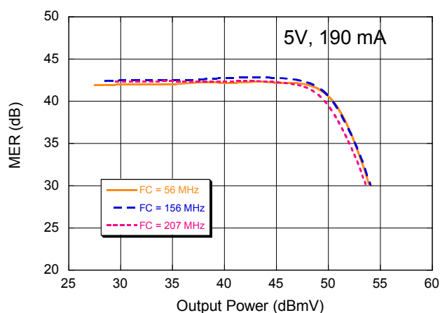
Modulation Error Ratio (64 QAM, 16 channel)
