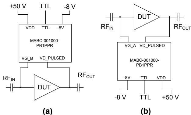
Figure 2. Pulsed Gate/Pulsed Drain Biasing: (b) North Biasing; (a) South Biasing
