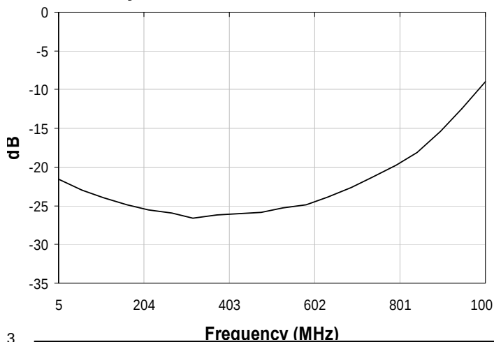
Directivity
