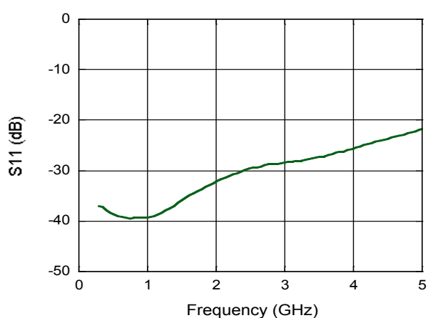
Input Return Loss, R_X
