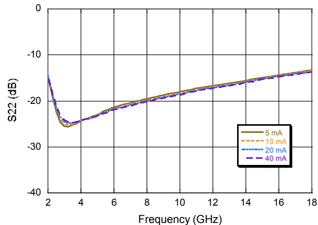
Output Return Loss @ 5 V, +25°C
