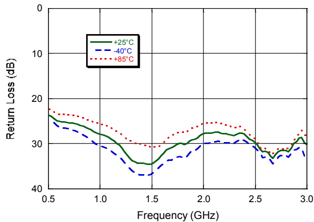
Return Loss
