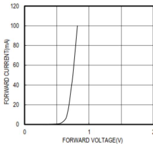
FORWARD I-V CHARACTERISTICS
