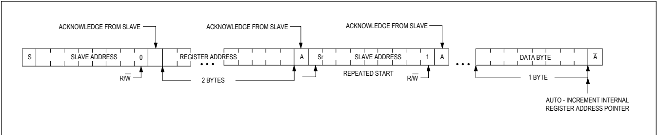
Figure 38. I 2 C Reading n-Bytes of Data from the Slave
