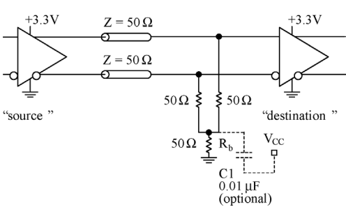
Figure 5. Three-Resistor “Y-Termination”
