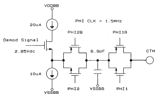
Figure 2 CTH Pin
