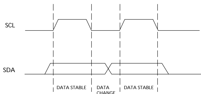
Figure 12: Data Validity
