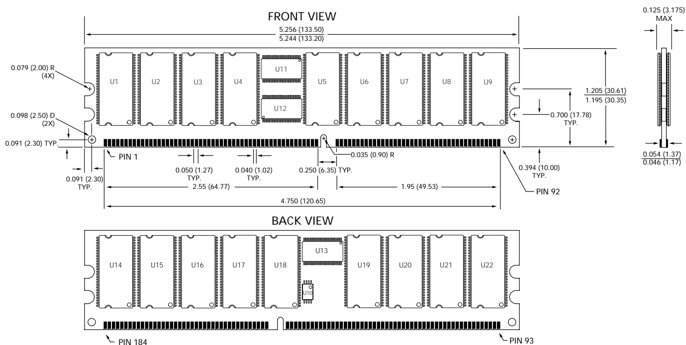
Figure 17: 184-Pin DIMM Dimensions (Low-Profile)
