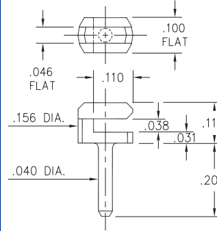
7310-0-01-XX-00-00-08-0 Board edge press-fit
