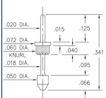
8816-0-00-XX-00-00-03-0 Press-fit in .057 mounting hole
