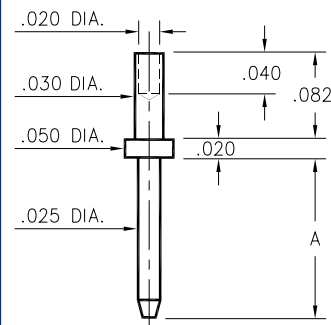
3120-X-00-XX-00-00-08-0 Swage mount in .034 mounting hole
