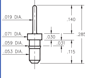
8876-0-00-XX-00-00-03-0 Press-fit in .057 mounting hole
