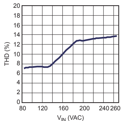
THD vs. V_{IN} @ Full-Load
