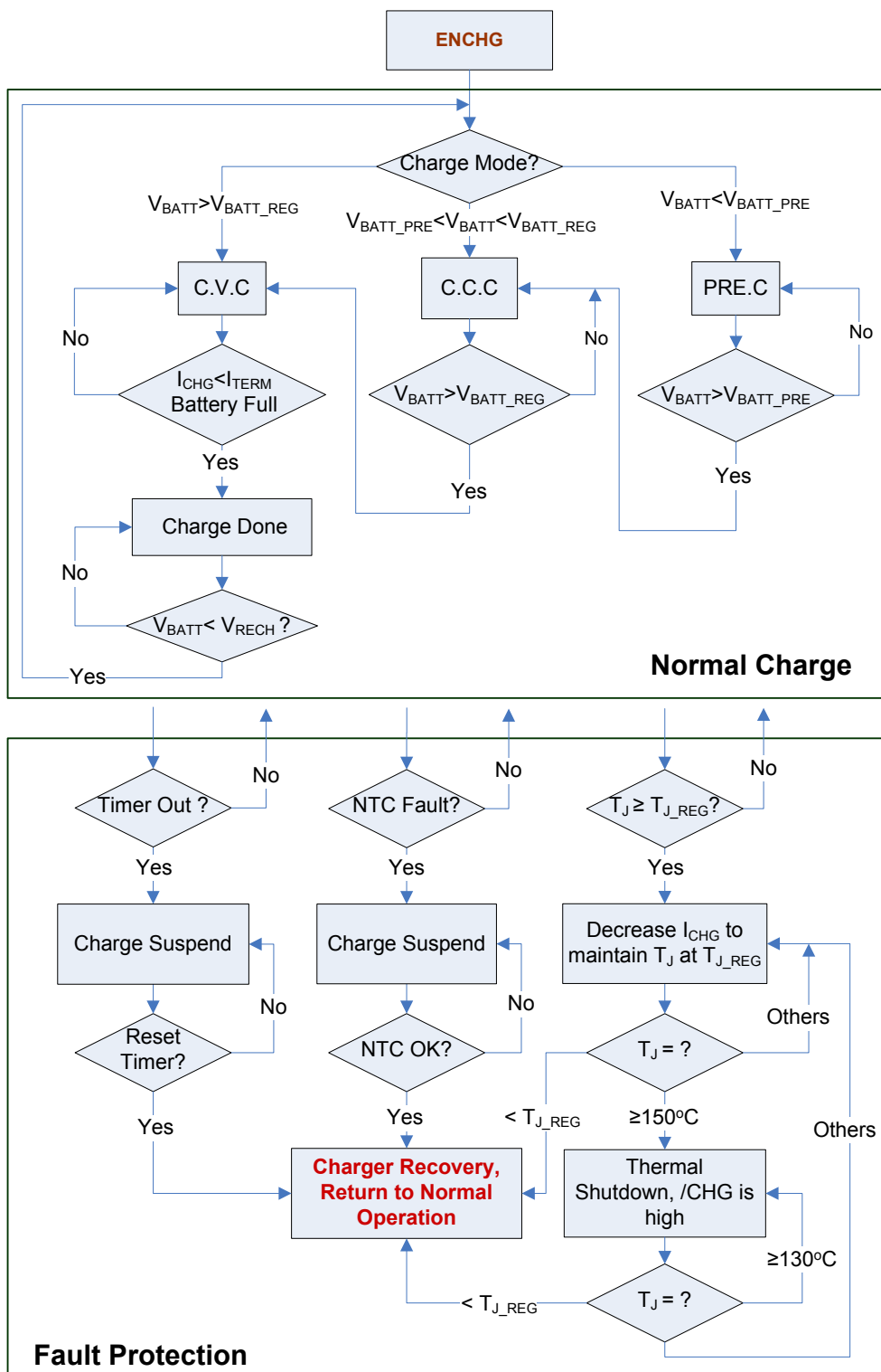
Figure 16: Charging Process
