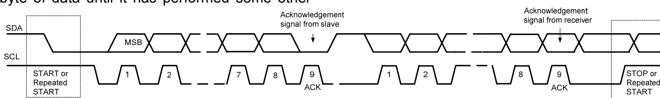
Figure 9: Data transfer on the I2C BUS
