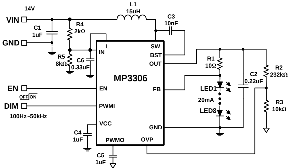
Figure 8— The application when V_{in} > 12V
