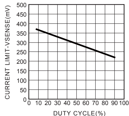
Figure 3— V_{SENSE} vs Duty Cycle
