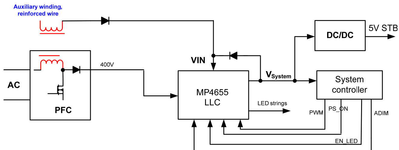
Figure 10: LLC Power System without External Standby Flyback
