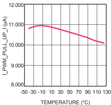
PWM Pull Up Current vs. Temperature
