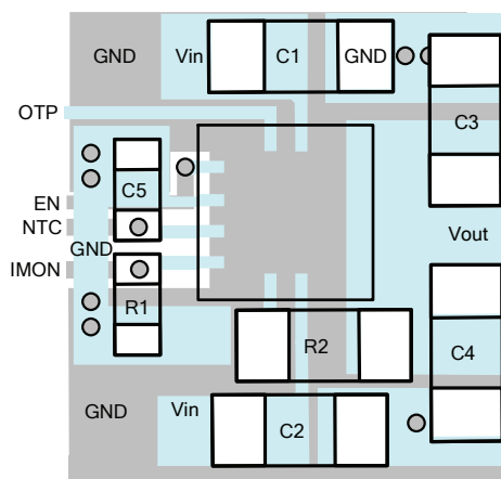
Figure 6: Recommended Layout
