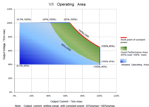
V/I Curve
