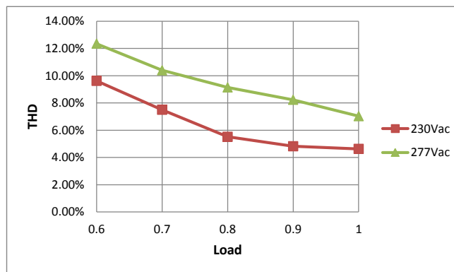
THD Curve
