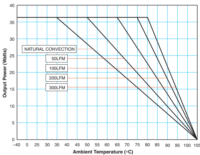
UNR-2.5/15-D5 Output Power Derating vs. Ambient Temperature
