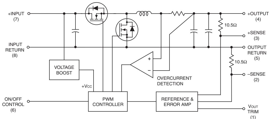
Figure 1. Simplified Schematic
